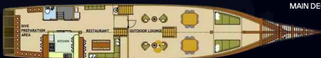
MAIN DECK
