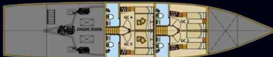
LOWER DECK
